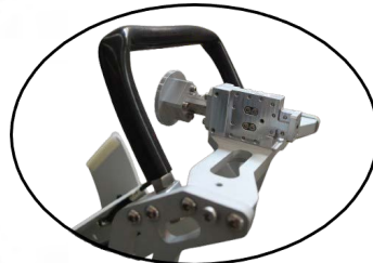
2 Port Q-band feed option
